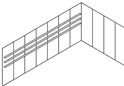
10 W358.25/204.75 D0.75/4.75 H117.17"
