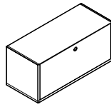
AS03 Cupboard Top W900 D380 H400 mm
