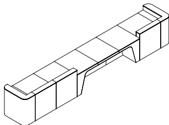
6 W5600 D875 H750/900/1100 mm
